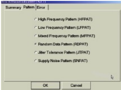
Figure 10: Layer 1 BERT patterns
